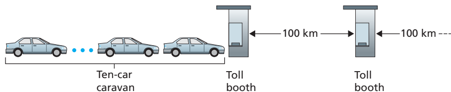
Figure 1.17 ♦ Caravan analogy
