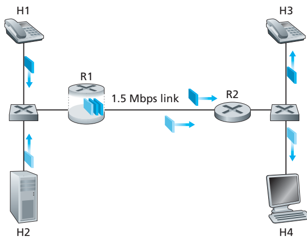
Figure 7.14 ♦ Competing audio and HTTP applications
